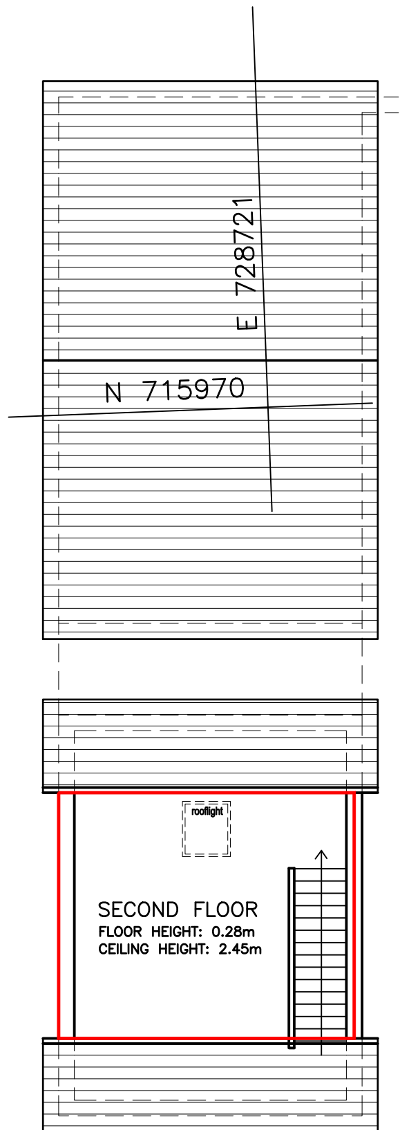
SECOND FLOOR PLAN (1:100)
